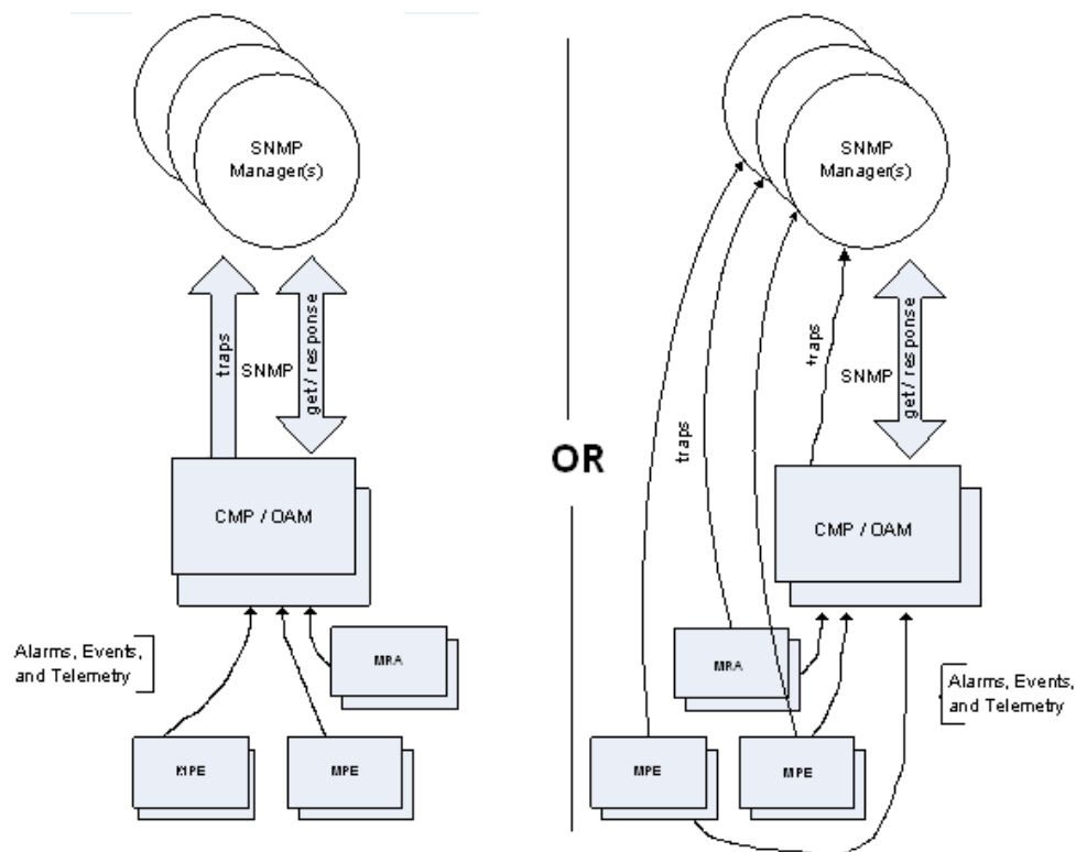
Figure 2-1 SNMP Configuration
